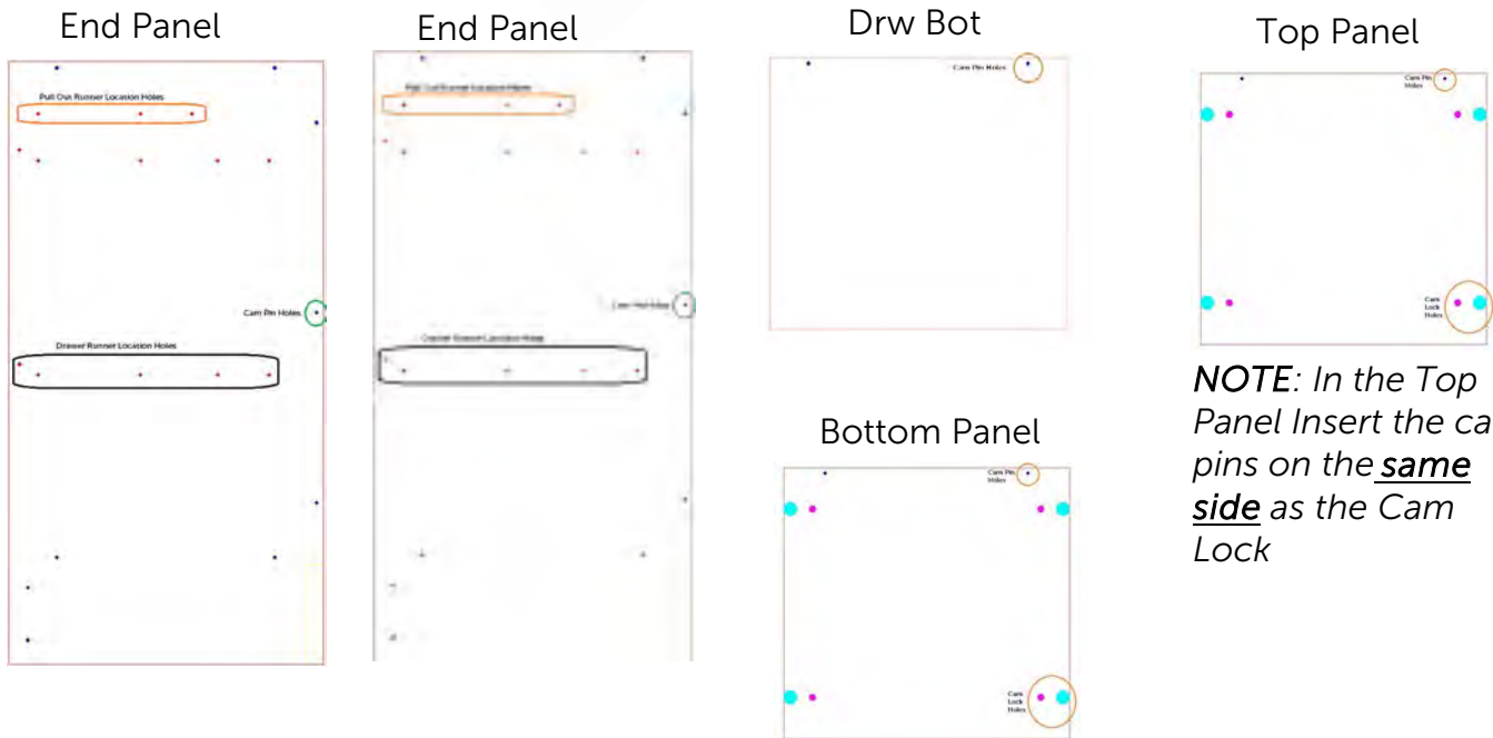
Pull Out Drawer /Table Front
